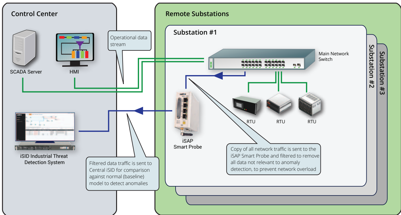
Deployment of a central iSID Industrial Threat Detection System using iSAP Smart Probes at remote sites
