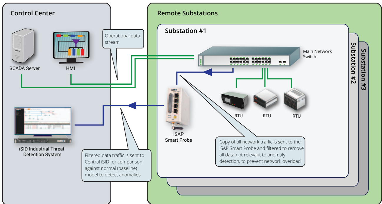
Deployment of a central iSID Industrial Threat Detection System using iSAP Smart Probes at remote sites
